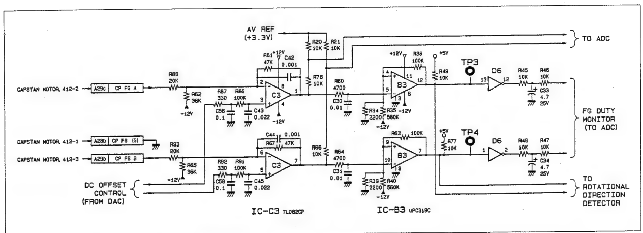
Fig. 4-3-7. Capstan FG Interface (CD-35 Board)
